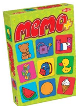
MEMO+ saker 01503
